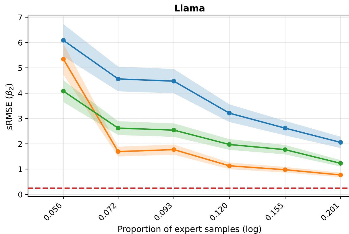
Low-Variance Feature — sRMSE \beta_2 with LLM baseline (MISOGYNISTIC)
